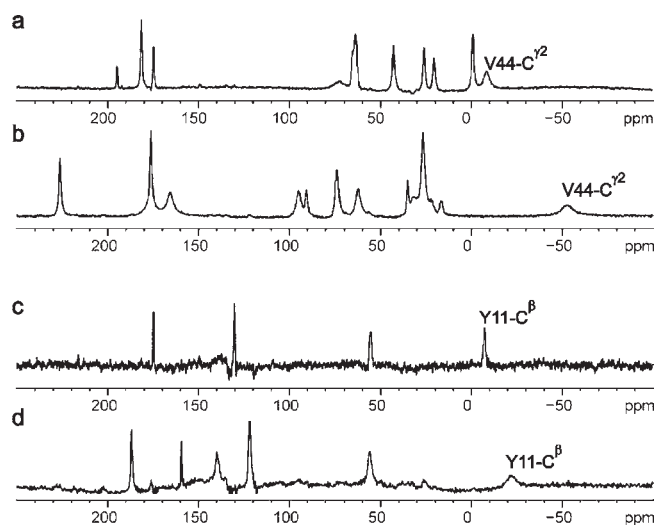
Figure 1. Example of selective labeling used in assigning the ^{13}\text{C} NMR signals from Clostridium pasteurianum rubredoxin with anomalous chemical shifts. (a) Reduced rubredoxin labeled with [U- ^{13}\text{C} ]-valine. (b) Oxidized rubredoxin labeled with [U- ^{13}\text{C} ]-valine. (c) Reduced rubredoxin labeled with [U- ^{13}\text{C} ]-tyrosine. (d) Oxidized rubredoxin labeled with [U- ^{13}\text{C} ]-tyrosine. The data collection method was optimized such that signals from nuclei close to the Fe–S center were observed preferentially in these spectra. The annotated ^{13}\text{C} signals have unusual chemical shifts when compared to the diamagnetic averages obtained from BMRB. 19 We attribute these large shifts to participation of these carbons and their attached hydrogens in 3c–4e interactions with sulfur atoms coordinated to iron: \text{CH}\cdots\text{S}\text{--Fe} .
