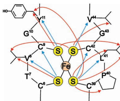
Figure 3. Schematic representation of hydrogen bonds and 3c–4e interactions at the active site of Clostridium pasteurianum rubredoxin. The \text{C}-\text{H}\cdots\text{S} 3c–4e interactions reported here (red arrows) were detected by 3c–4e Fermi-contact shifts on ^{13}\text{C} . The \text{N}-\text{H}\cdots\text{S} hydrogen bonds (blue arrows) were detected previously 31 by trans-hydrogen-bond Fermi-contact effects on ^{15}\text{N} chemical shifts.
